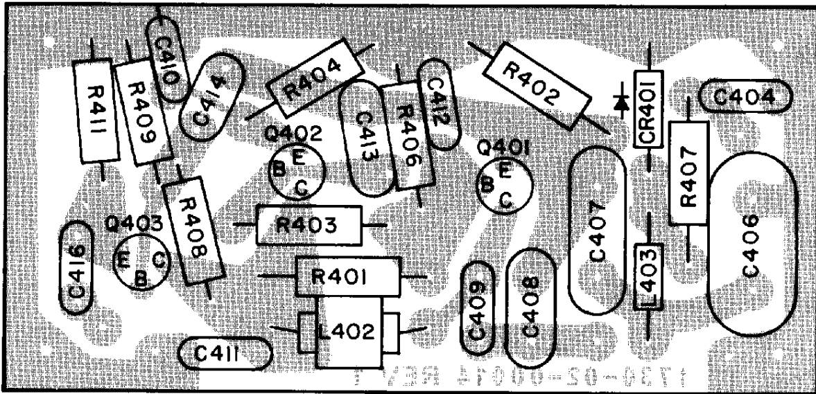
FIGURE 7-3 X-RAY VIEW, VFO MODULE
