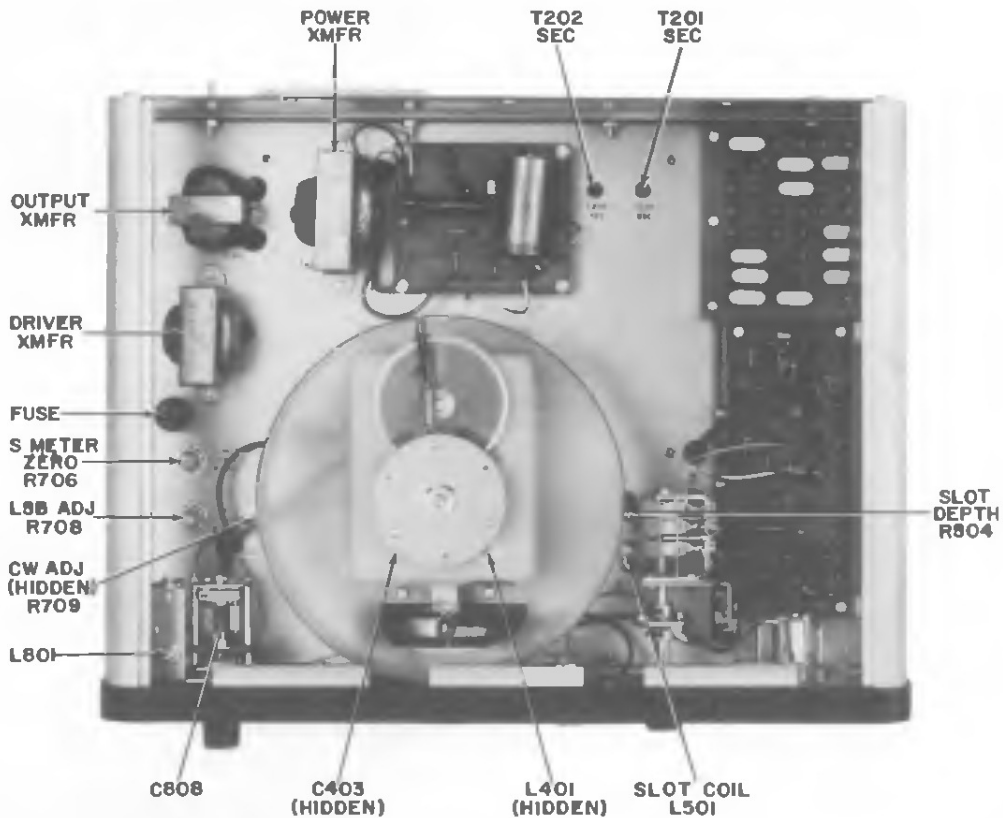
FIGURE 4-1 TOP VIEW OF HQ-215
