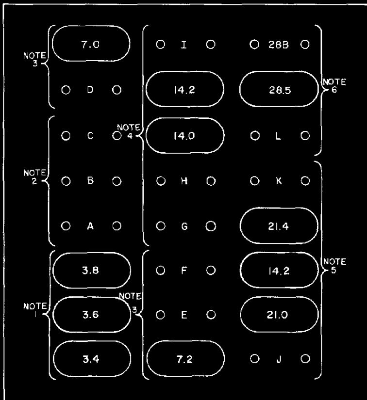
FIGURE 2-2 CRYSTAL LOCATION
