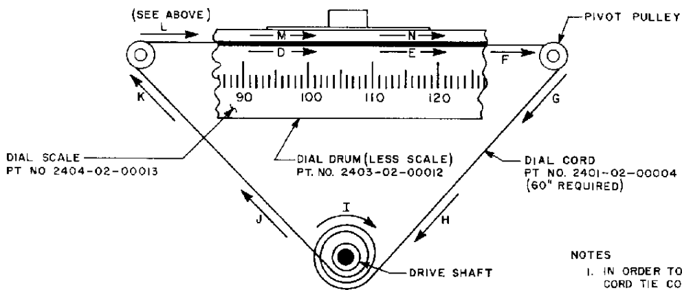
VIEW THRU FRONT PANEL
